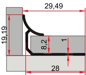
MP 255 C 0,142 kg/m Fayans İ Köşe 8 Luk 8 MM CERAMIC COVER PROFILE INNER
