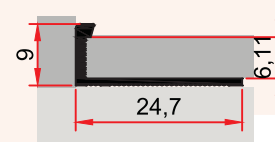
ST 250 B 0,103 kg/m 8 lik Basamak Burunluđu 8 MM STEPNOSE PROFILE
