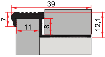
ST 253 D 0,173 kg/m Basamak Burunluđu STEPNOSE PROFILE
