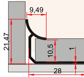
MP 255 D 0,149 kg/m Fayans İ Köşe 10 Luk 10 MM CERAMIC COVER PROFILE INNER
