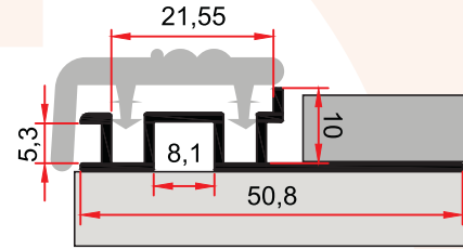
ST 253 B 0,259 kg/m 10 mm. Fitilli Basamak Burunluđu STEPNOSE PROFILE WITH WICK
