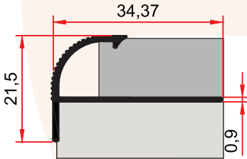
ST 255 0,184 kg/m Basamak Burunluđu STEPNOSE PROFILE
