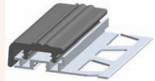
ST 253 0,257 kg/m Basamak Burunluđu STEPNOSE PROFILE
