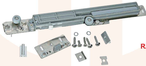
1075 RAY İÇİ YAVAŞLATICI ÇİFT PİSTONLU 1075 FAIR TO SLOW DOWN THE DOUBLE-PISTON
