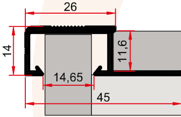
ST 253 A 0,289 kg/m Basamak Burunluđu STEPMOSE PROFILE
