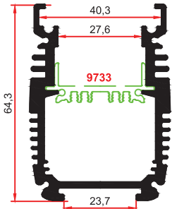
7494 1,540 Kg/m
