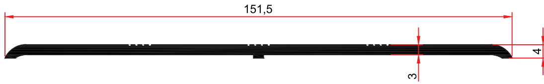
ST 224 F 1,210 kg/m
