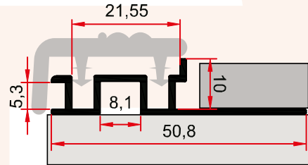
ST 253 B 0,259 kg/m 10 mm. Fitilli Basamak Burunluđu STEPMOSE PROFILE WITH WICK
