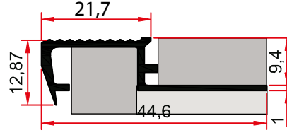
ST 253 0,257 kg/m Basamak Burunluđu STEPMOSE PROFILE
