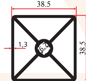
SK 709 1,020 Kg/m
