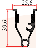
9188 LED AYAĞI 0,585 Kg/m
