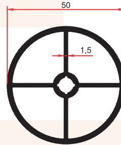
SM 5011 C 1,240 Kg/m
