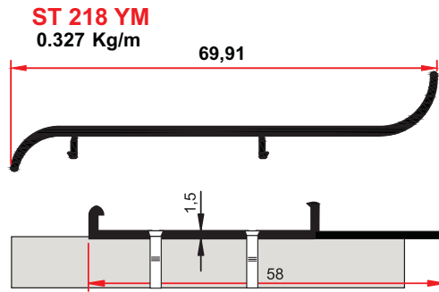
ST 218 YM ALT ST 218 YM BOTTOM PVC ( 80 mm boyda - ADET )
