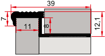
ST 253 D 0,173 kg/m Basamak Burunluđu STEPMOSE PROFILE
