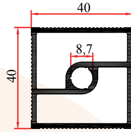
SK 702 1,105 Kg/m
