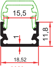
LED PROFİL KAPAK 9029-1
