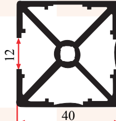
SK 5009 A 1,210 Kg/m
