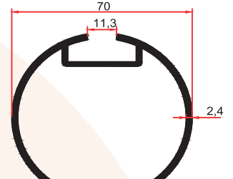
SM 5017 1,525 Kg/m
