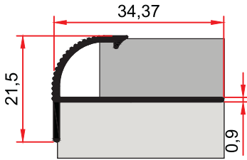
ST 255 0,184 kg/m Basamak Burunluđu STEPMOSE PROFILE
