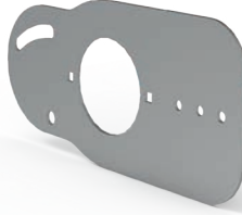
Arka Ray Deliksiz Saç Rail Back sheet without hole PRG-02-10400-34-0X
