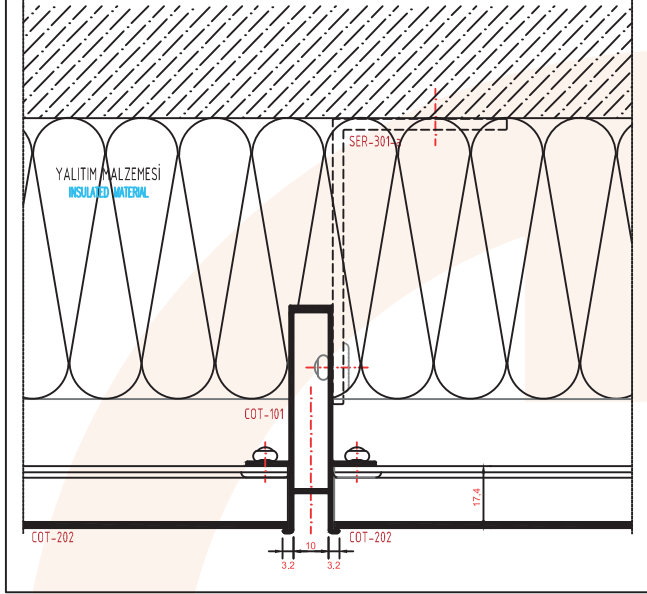
PLAN DETAY PLAN DETAIL
