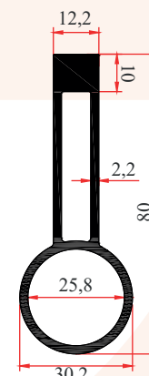
PRF-30538 1,340 Kg/m
