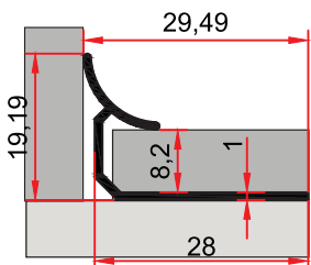
MP 255 C 0,142 kg/m Fayans İç Köşe 8 Lik 8 MM CERAMIC COVER PROFILE INNER
