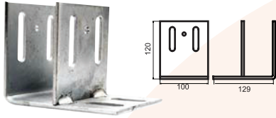
F Tipi Cephe Ankraji F Type Facade Anchor
