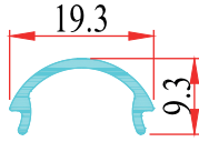
LED PROFİL KAPAK 9029-2
