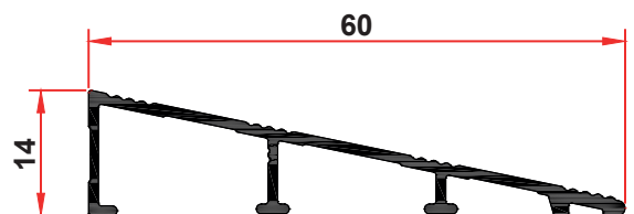
PRF-30419 0,300 Kg/m
