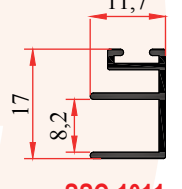
SSC-1011 0,120 Kg/m CAM FİTİLLİ ALM-8MM
