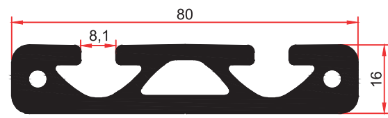
FS 4021 2,240 Kg/m
