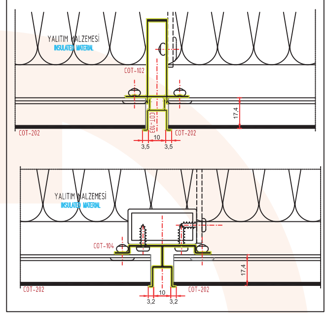
PLAN DETAY PLAN DETAIL
