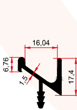
5981 A 0,300 Kg/m
