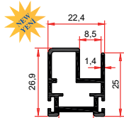
PRF-30109 0,475 K g/m
