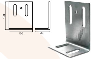
L Tipi Cephe Ankraji L Type Facade Anchor
