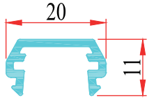
LED PROFİL KAPAK 9029-1
