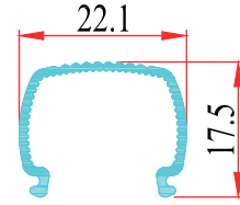
LED PROFİL KAPAK 9029-4
