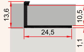
ST 250 E 0,122 kg/m 12 lik Basamak Burunluğ 12 MM STEPNOSE PROFILE
