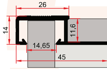
ST 253 A 0,289 kg/m Basamak Burunluđu STEPNOSE PROFILE
