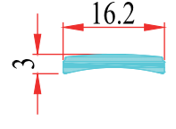
LED PROFİL KAPAK 9029-5
