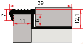
ST 253 D 0,173 kg/m Basamak Burunluđu STEPNOSE PROFILE
