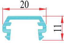
LED PROFİL KAPAK 9029-1
