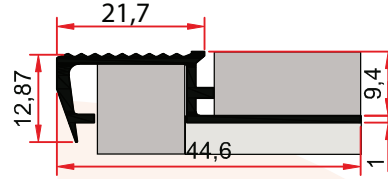
ST 253 0,257 kg/m Basamak Burunluđu STEPNOSE PROFILE
