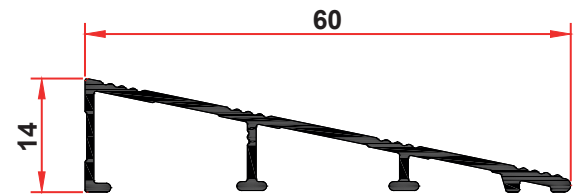
PRF-30419 0,300 Kg/m
