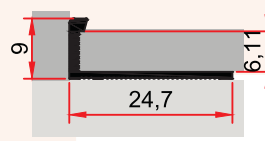
ST 250 B 0,103 kg/m 8 lik Basamak Burunluğ 8 MM STEPNOSE PROFILE
