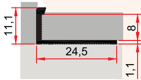
ST 250 D 0,111 kg/m 10 luk Basamak Burunluğ 10 MM STEPNOSE PROFILE
