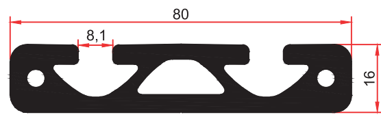
FS 4021 2,240 Kg/m
