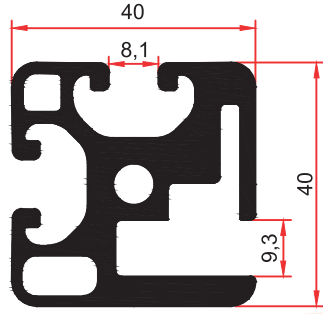
FS 4009 1,965 Kg/m
