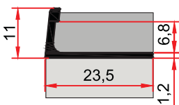
ST 250 0,124 kg/m Basamak Burunluğ STEPNOSE PROFILE
