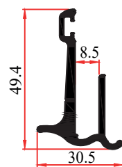
30138 8MM CAM APARATI 0,700 Kg/m
