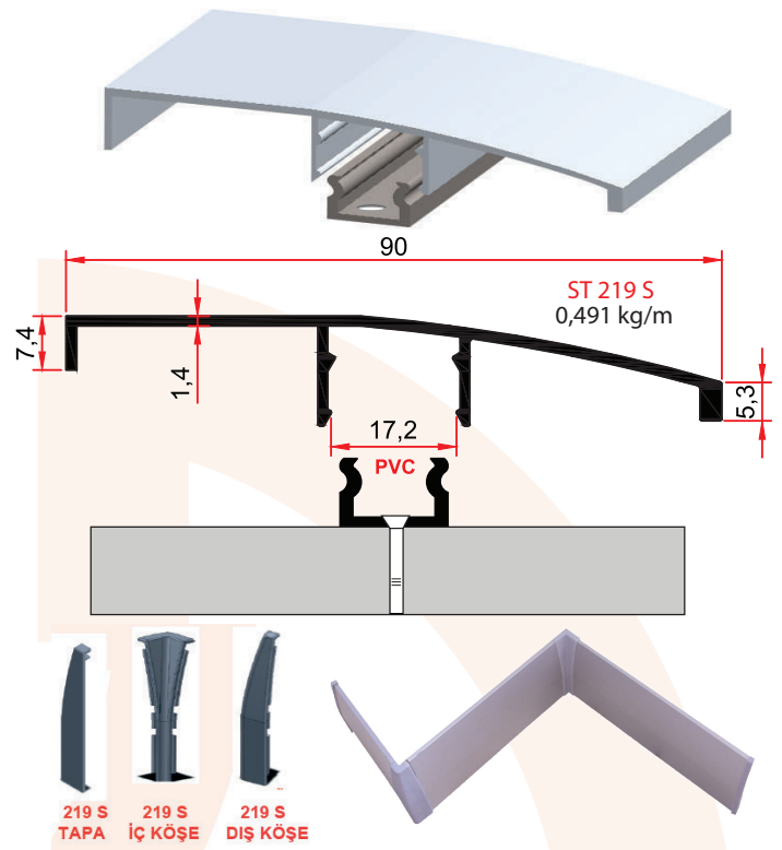
ST 219 S BASEBOARD INNER-OUTER CORNERS & PLUG
