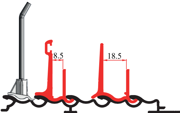
PRF-30139 1,080 Kg/m
