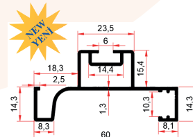
PRF-30671 0,586 Kg/m
