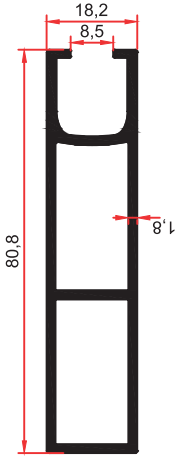
FS 4033 1,110 Kg/m
