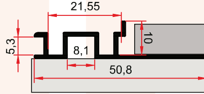
ST 253 B 0,259 kg/m 10 mm. Fitilli Basamak Burunluğu STEPPED PROFILE WITH WICK
